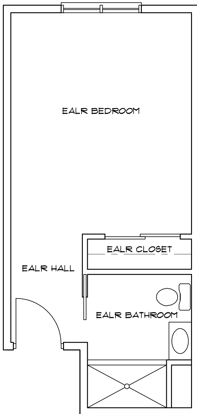
TYPICAL EALR UNIT SCALE: 1/4" = 1'-0"
