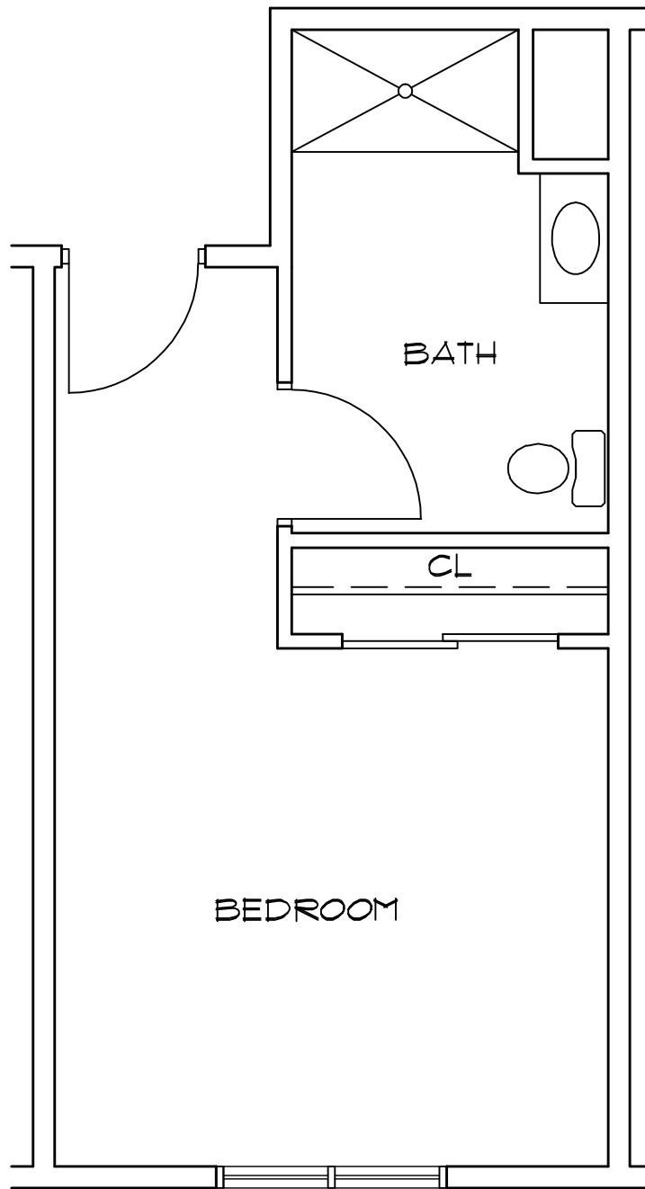
BEDROOM PLAN HC SCALE: 1/4" = 1'-0"
